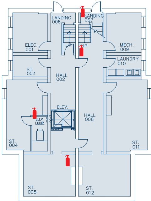
Basement
